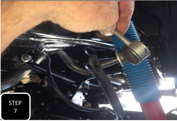
Step 7 Re-attach both sway bar end links and tighten.
